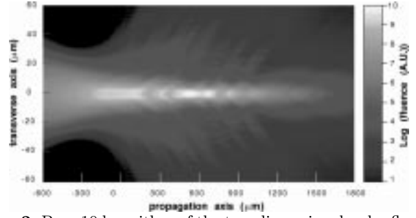
Fig. 2. Base 10 logarithm of the two-dimensional pulse fluence for a relativistic intensity of I = 3 \times 10^{18} W/cm 2 . Laser pulse propagates from left to right. The focal plane in vacuum corresponds to the position z = 0 . The peak fluence is 2.5 times the peak value in vacuum. Like in all the simulations presented here a cylindrical symmetry is assumed.
