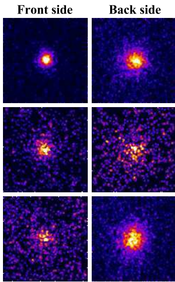
Figure 1: X-ray front and back pinhole camera images of the K shell emission obtained from the analysis of 350 data acquisitions. The target consisted of three layers: Cr( top ), Ni( center ) and Fe( bottom ).
