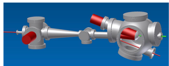
Figure 4: Final drawing of the Thomson scattering interaction chamber.
