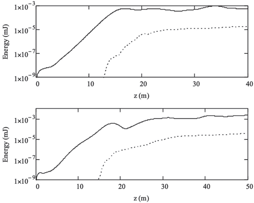
Fig. 24.5. Growth of the SASE FEL energy per pulse of Scheme 5-1 GeV (top) and Scheme 3-1 GeV (bottom) beam distributions for the short-undulator-period configuration. The fundamental (solid line) and third (dotted line) harmonics are shown.
