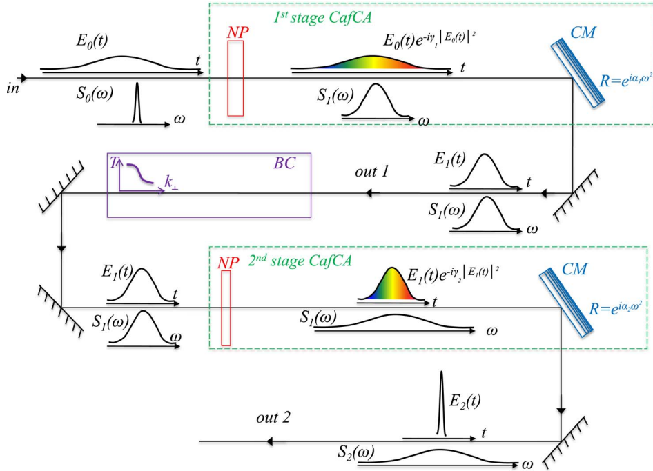
Figure 24. Diagram illustrating the Compression after Compressor Approach (CafCA) (NP – nonlinear plate, CM – chirped mirror, BC – beam cleaner: pinhole spatial filter [173] or free-space propagation [174] ).
