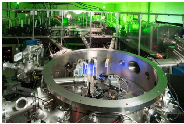
Figure 6. The Advanced Beam Laboratory at Colorado State University (picture courtesy of Colorado State University).
