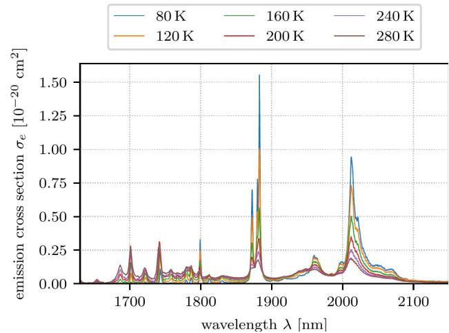
Figure 36. Temperature-dependent emission cross-sections of Tm:YAG.
