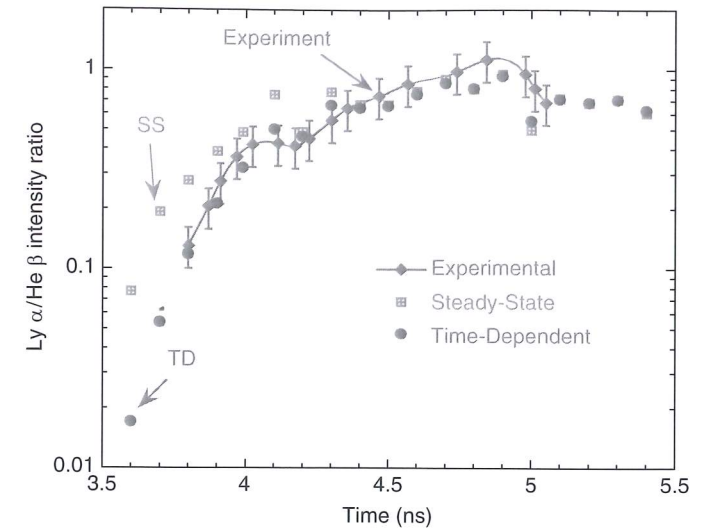
Fig. 10.21 Temporal evolution of Ly \alpha to He \beta intensity ratio. Experiment vs. steady-state (SS) and time-dependent (TD) modeling
