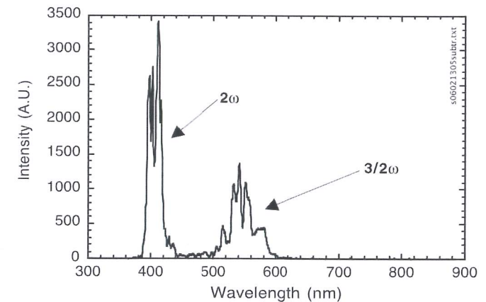
Fig. 10.8 Spectrum of optical scattering from laser interaction of a 60 fs laser pulse at an intensity of 10^{19} W/cm 2 with a 12- \mu m thick solid target. The spectrum was taken with a spectrometer capable of resolving the entire visible range, showing simultaneously the 2\omega and the (3/2)\omega emission components
