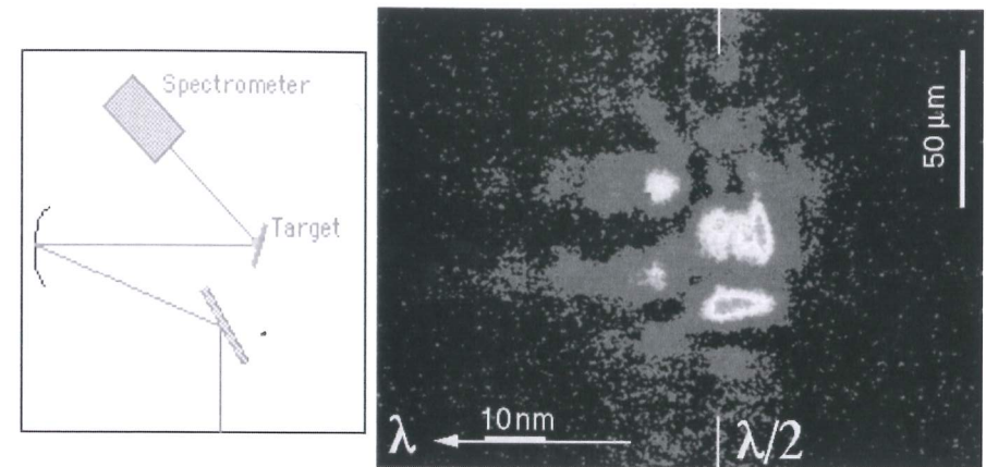
Fig. 10.7 Space-resolved spectrum of specular 2\omega emission from the interaction of a 35 fs laser pulse at an intensity of 5 \times 10^{18} W/cm 2 with a 1- \mu m thick plastic target. The intensity of the ASE was 10^{12} W/cm 2 , i.e., sufficiently high to lead to premature plasma formation. The spectrum shows a very broad (spectrally) and large (spatially) emission with complementary red- and blue-shifted components
