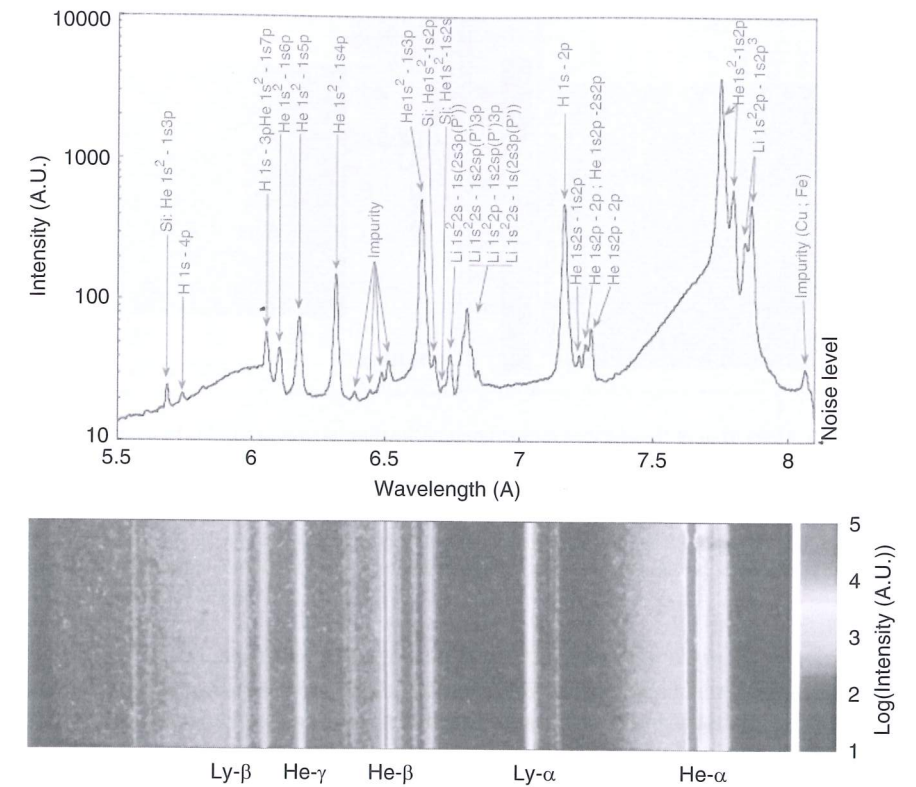
Fig. 10.19 Example of spectrum obtained using the setup of Fig. 10.18 from a plasma produced by laser irradiation of a solid Al target. Due to the small source size, the resolution is sufficiently high to allow identification of K-shell emission from helium-like and hydrogen-like aluminum
