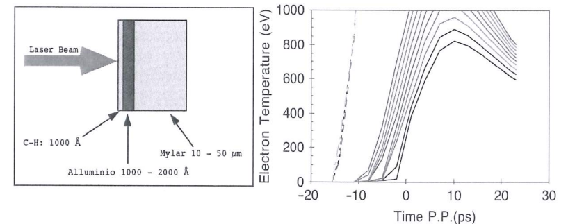
Fig. 10.24 (left) Target configuration for mass ablation rate measurements in intense laser–solid interactions [from [46]]. The aluminum tracer layer is used to detect propagation of the ablation front. Numerical modeling (right) is used to calculate the expected evolution of the electron temperature to be compared with experimental measurements via time-resolved spectroscopy
