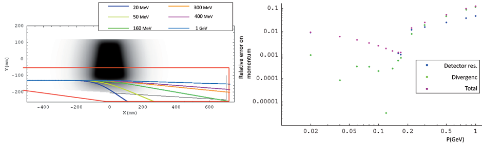
Fig. 1. – (Colour on-line) Left: working principle of the of the SITE spectrometer. The black area represents the area with magnetic field directed orthogonally to the picture. Also shown are the trajectories of the particles (colour lines), the locations of the position detectors (black lines), and the contour of the vacuum chamber (red line). Right: expected resolution showing the error originating from the position resolution of the detector and the error due to the beam divergence.
