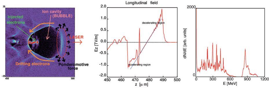
Fig. 2. – The bubble regime. Left: plot of the electron density; middle: line-out of the longitudinal field along the bubble axis. Right: energy spectrum of the accelerated electrons as obtained from the 3D PIC simulation for the SITE after a propagation of 4 mm inside the gas-jet.
