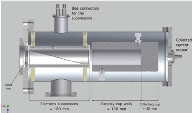
Fig. 9.11 Schematic layout of a Faraday Cup detector. The current collected in the cup is sent to an electrometer for integration. Figure credit: [26]
