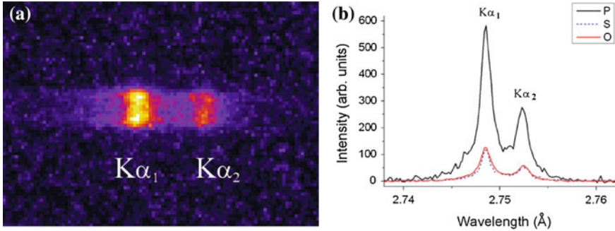
Fig. 8.3 a Raw spectrum of fluorescence Ti K- \alpha emission from laser irradiation of a Ti foil at moderately relativistic intensity ( a_0 \simeq 1 ), obtained by averaging 100 p-polarized laser pulses. b Ti K- \alpha spectra obtained by different laser pulse polarizations, and obtained by averaging 100 laser shots (after [34])
