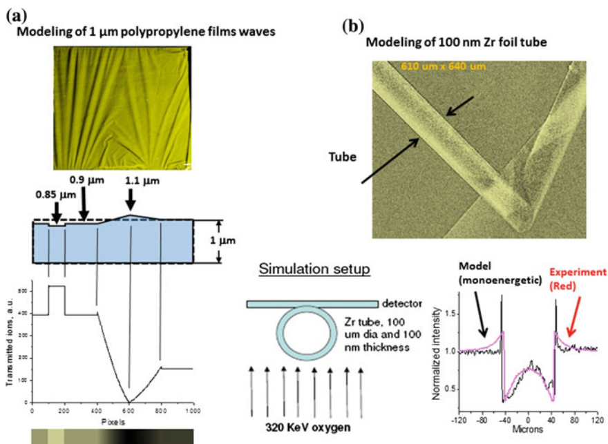
Fig. 12.7 The simulations ( bottom ) for the case a of 1 \mu\text{m} polypropylene foil waves was performed with 250 keV carbon ions [82–84]. Clear steps on the image correspond to variations of polypropylene thickness of 100–150 nm; for the case b of 100 nm Zr foil tube simulation was performed with 320 keV oxygen ions
