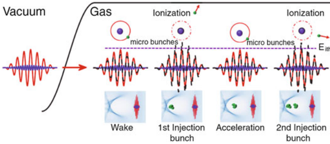
Fig. 7.4 Schematic view of dual color lasers triggered periodic injection in LWFA. A laser with base frequency \omega_1 (the red curves) and its harmonic \omega_2 (the blue curves) propagate in a mixed gas plasma. The dashed black curves show the superposition of the two frequency laser fields at different propagation distances. Laser parameters are chosen so that ionization-induced injection can be switched on when the beating is constructive and be switched off when the beating is destructive. In the plot, E_{ith} represents the effective threshold field for the high-Z gas inner shell ionization. Reprinted figure with permission from Zeng et al. [15]. Copyright (2015) by the American Physical Society
