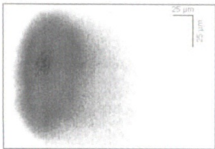
FIGURE 6. X-ray image of the interaction of a 12-ps laser pulse focused to a \approx 25\text{-}\mu\text{m} focal spot on a solid Al target at an intensity of \approx 10^{17} \text{ W/cm}^2 .
